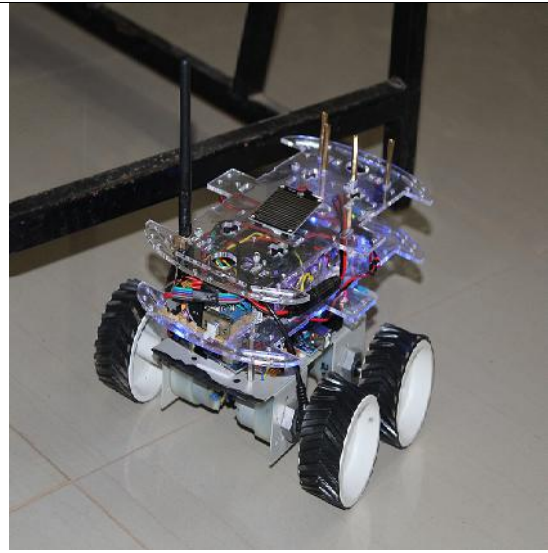
Multifunction Smart Bot designed and developed by the student
